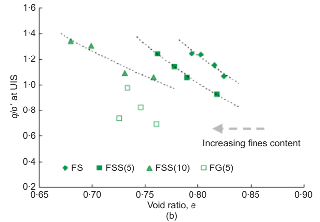
Fig. 18. Variation of stress ratio at undrained instability with void ratio: (a) mixtures with Toyoura sand as host sand; (b) mixtures with Fujian sand as host sand
